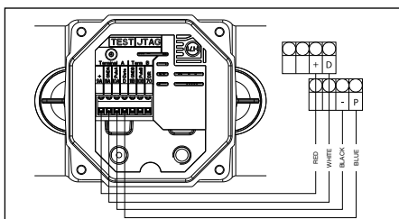
Connection AXONIC/C800
