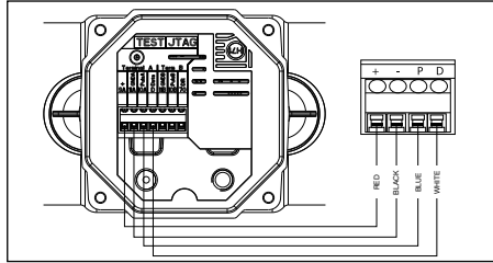
Connection AXONIC/CF51-CF55-Pulse-Box
